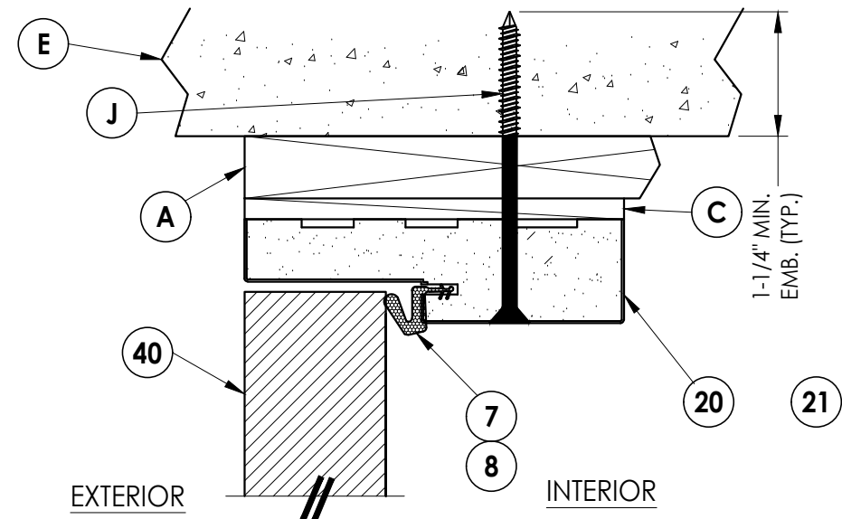
2 VERTICAL CROSS SECTION 6 Outswing shown - inswing also approved Shown w/1X sub-buck
