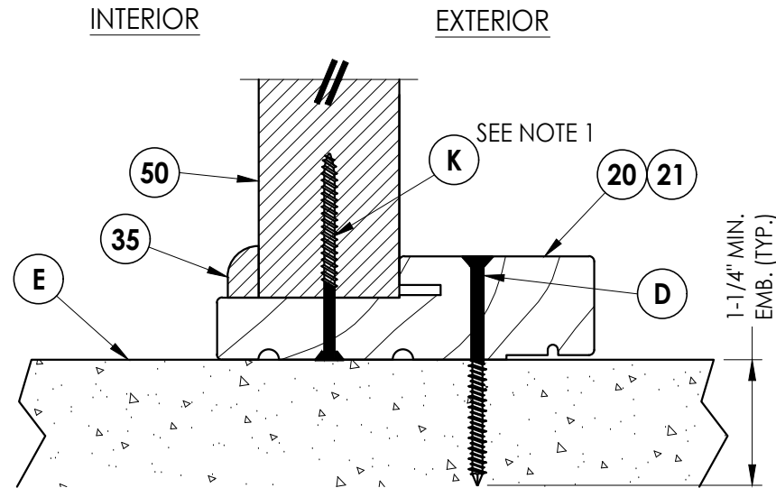
5 7 VERTICAL CROSS SECTION Outswing configuration
