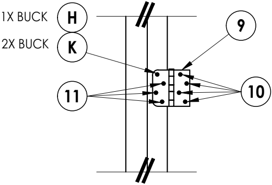
HINGE DETAIL
