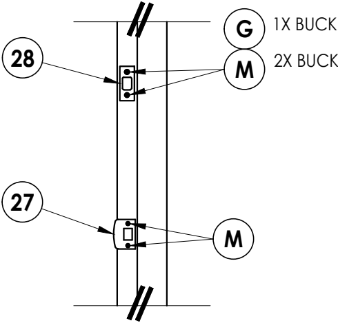
LATCH & DEADBOLT DETAIL
